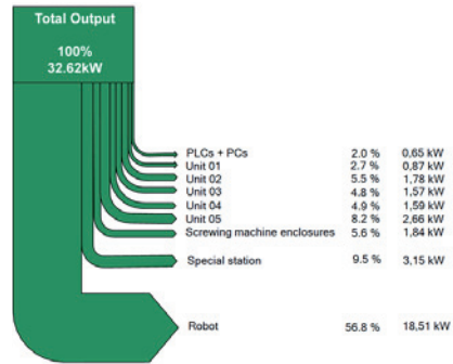
Energy demand distribution in a 'typical' cell
